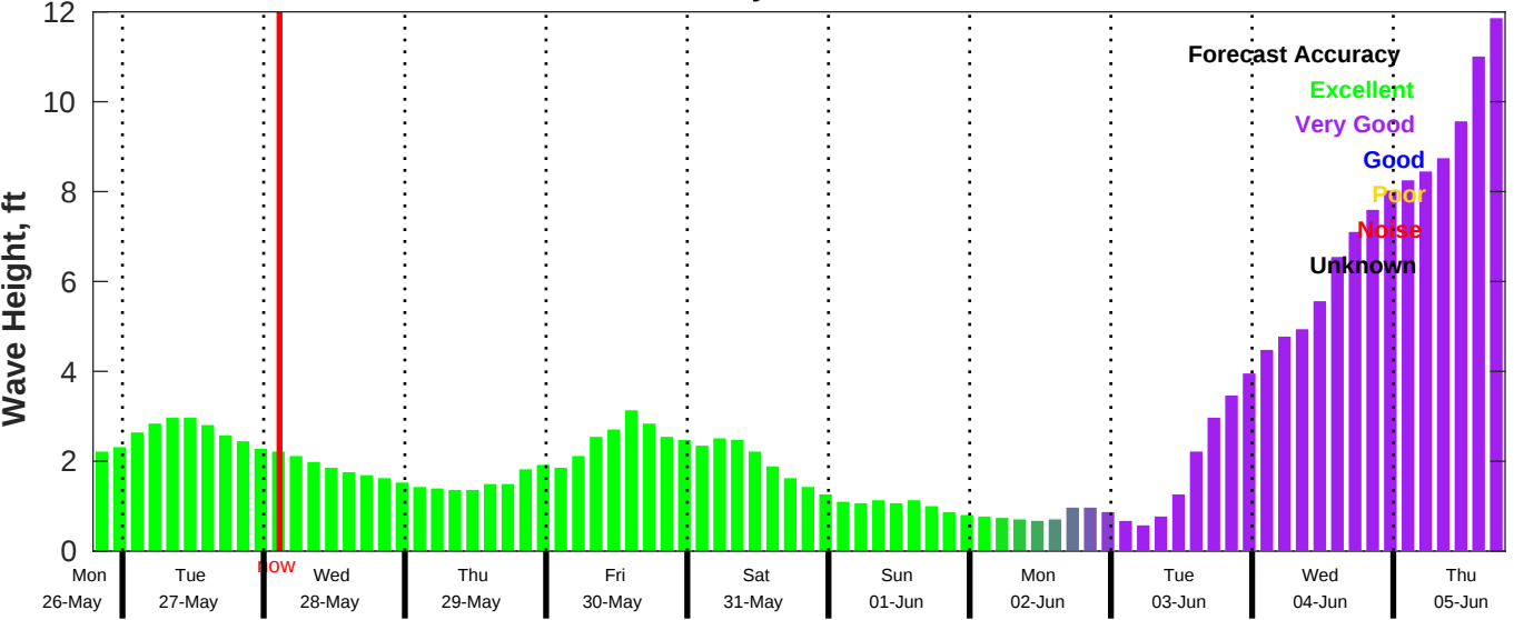
CMEMS Wave Forecast for NDBC 42040 from 26-May-2025 19:00:00 to 05-Jun-2025 19:00:00
