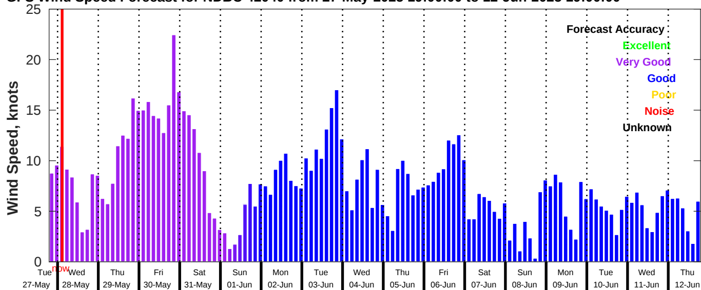
GFS Wind Speed Forecast for NDBC 42040 from 27-May-2025 19:00:00 to 12-Jun-2025 19:00:00
