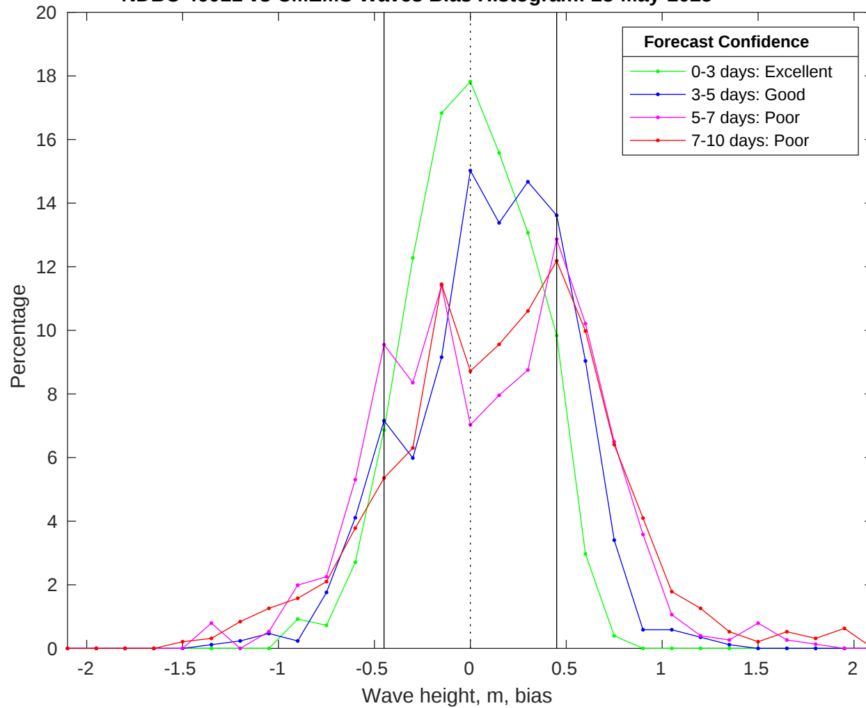
NDBC 46011 vs CMEMS Waves Bias Histogram: 28-May-2025
