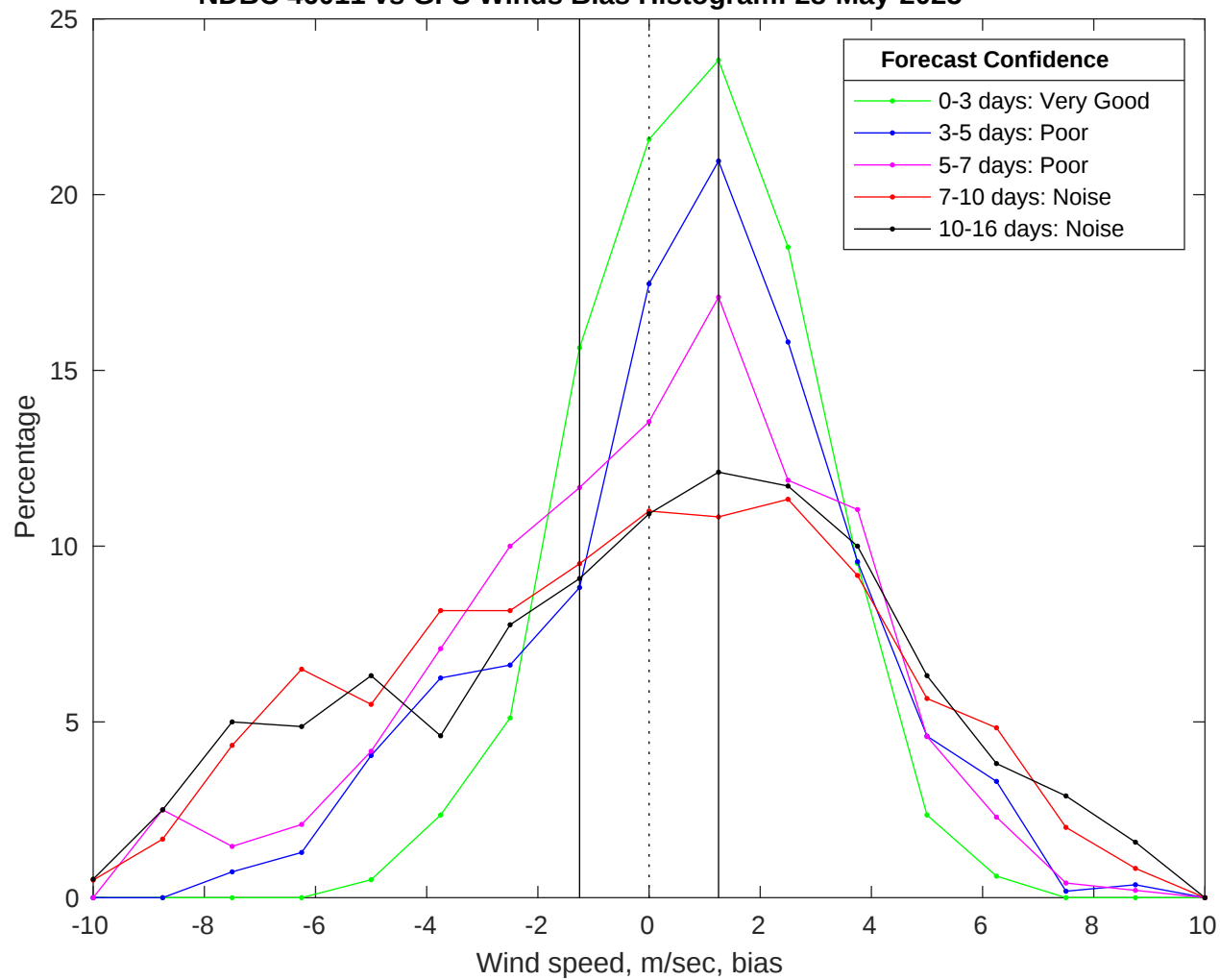
NDBC 46011 vs GFS Winds Bias Histogram: 28-May-2025
