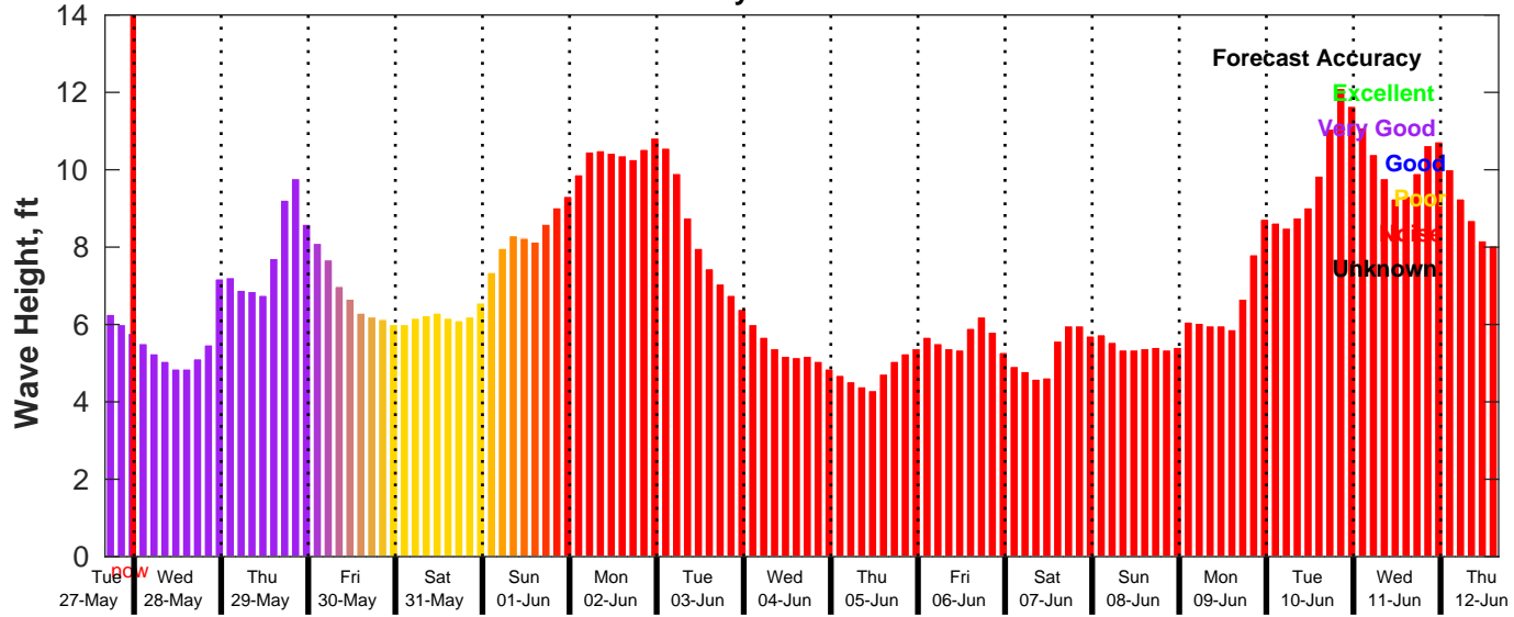
GFS Wave Forecast for NDBC 46011 from 27-May-2025 16:00:00 to 12-Jun-2025 16:00:00
