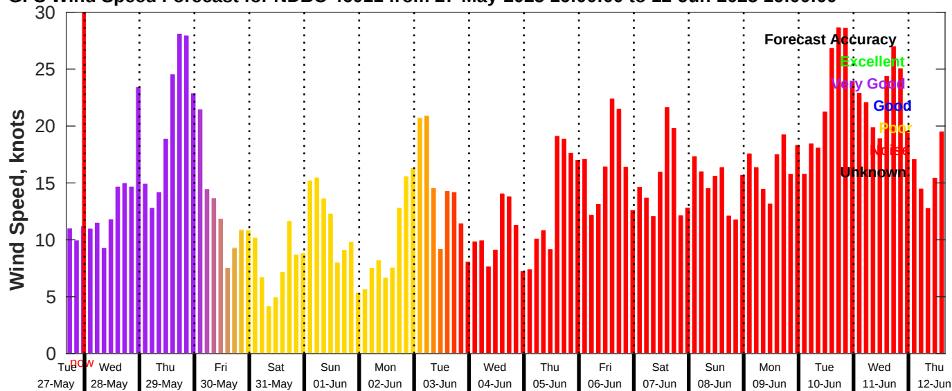
GFS Wind Speed Forecast for NDBC 46011 from 27-May-2025 16:00:00 to 12-Jun-2025 16:00:00
