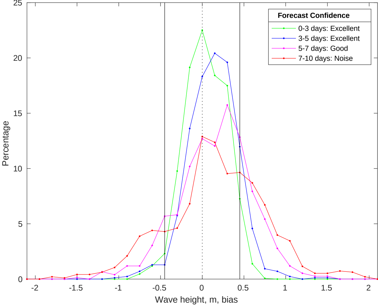
NDBC 46028 vs CMEMS Waves Bias Histogram: 28-May-2025
