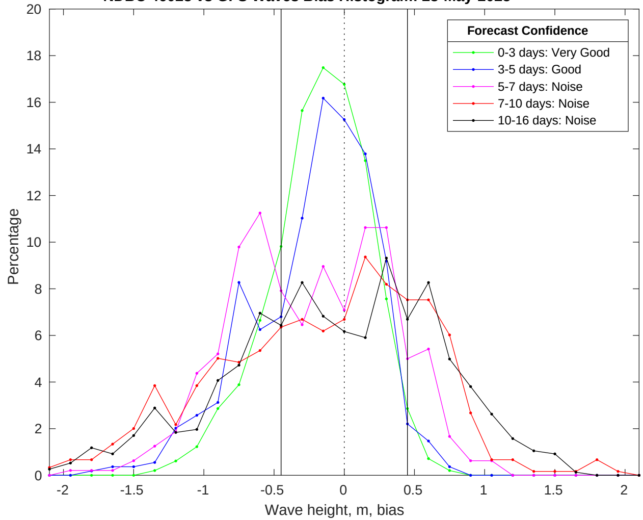
NDBC 46028 vs GFS Waves Bias Histogram: 28-May-2025
