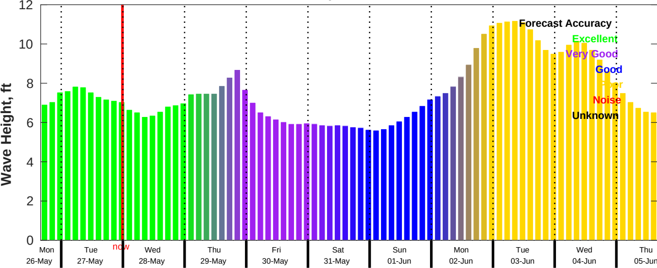
CMEMS Wave Forecast for NDBC 46054 from 26-May-2025 16:00:00 to 05-Jun-2025 16:00:00
