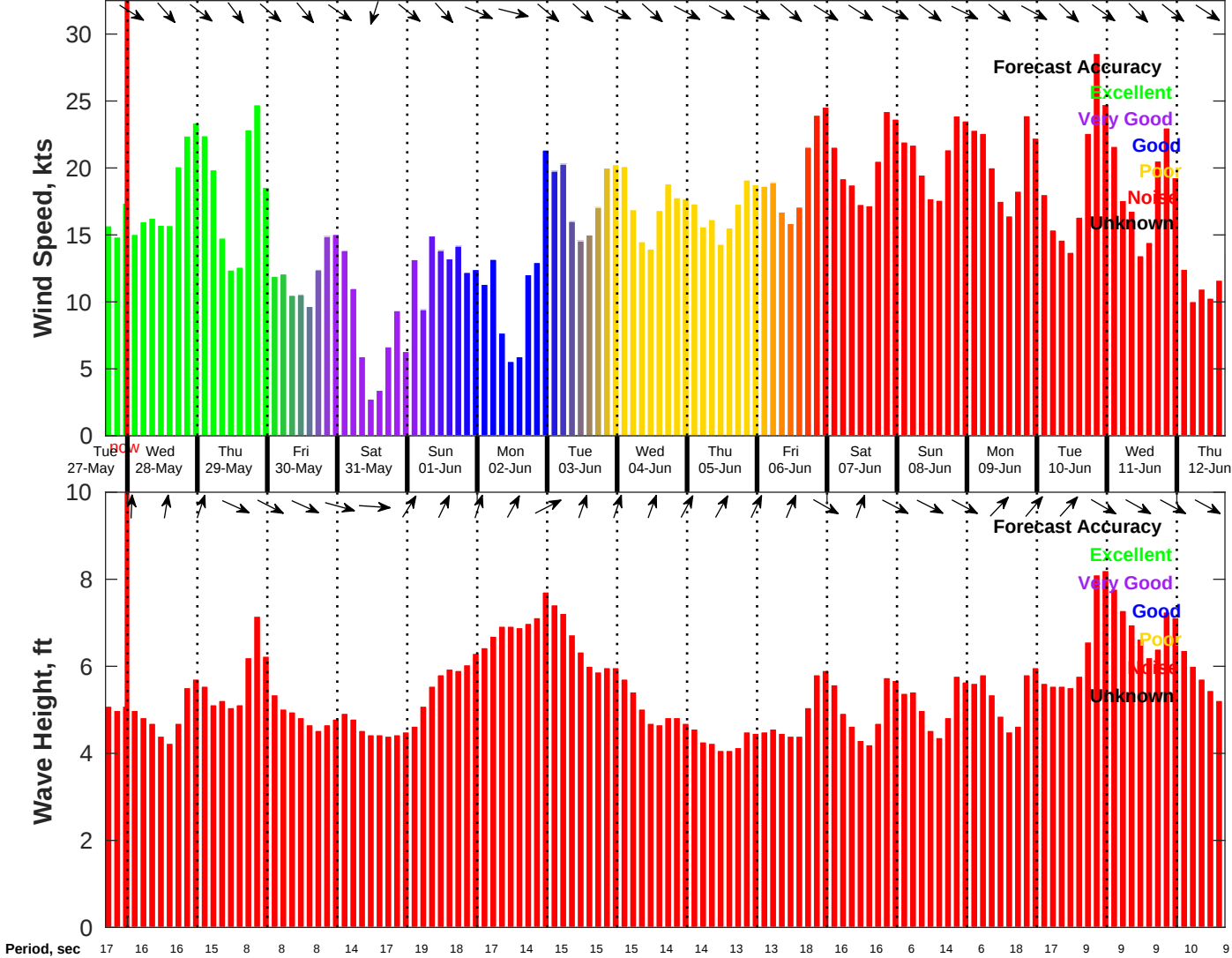
Wind & Wave Forecast for NDBC 46069 from 27-May-2025 16:00:00 to 12-Jun-2025 16:00:00
