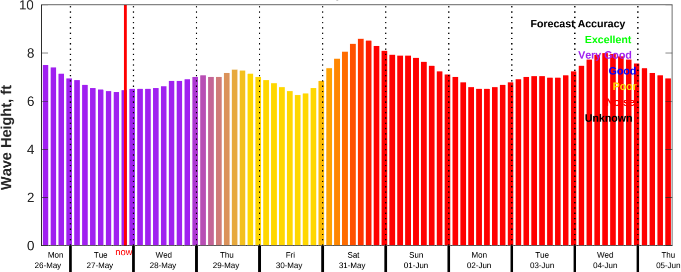
CMEMS Wave Forecast for NDBC 51209 from 26-May-2025 13:00:00 to 05-Jun-2025 13:00:00
