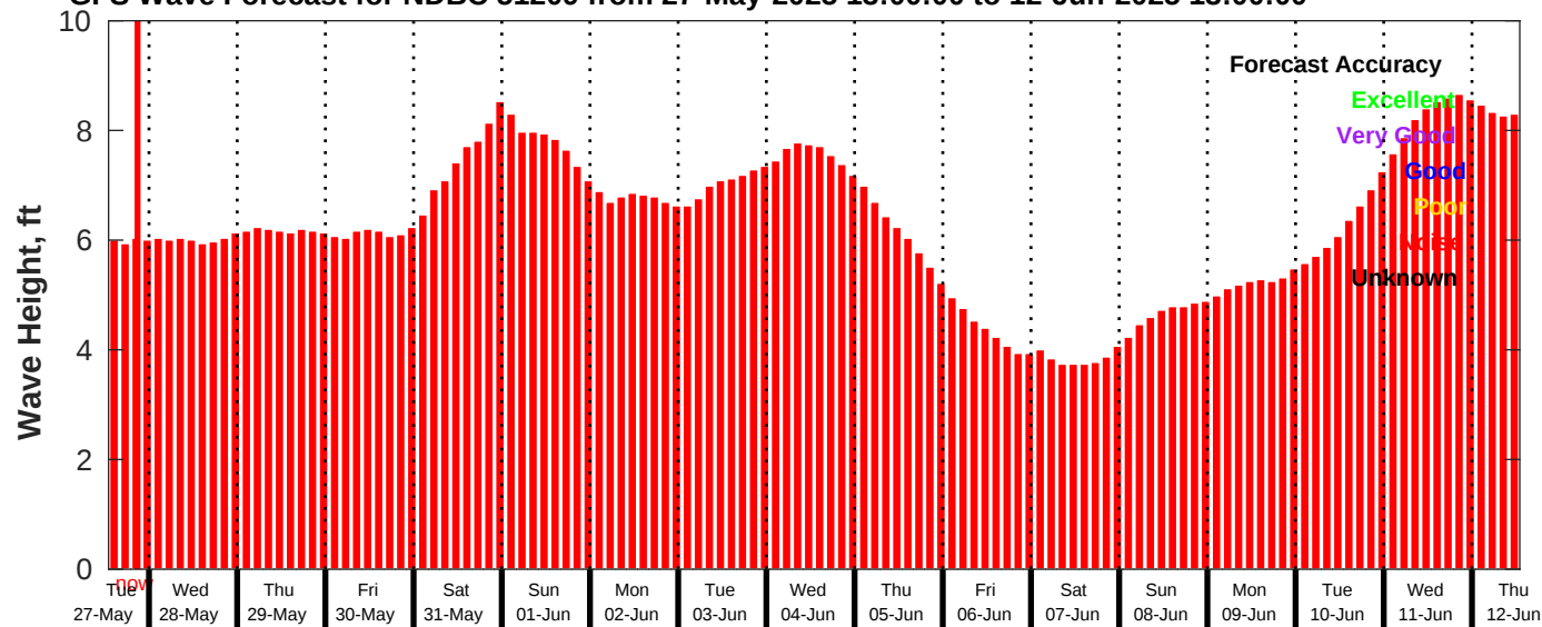
GFS Wave Forecast for NDBC 51209 from 27-May-2025 13:00:00 to 12-Jun-2025 13:00:00
