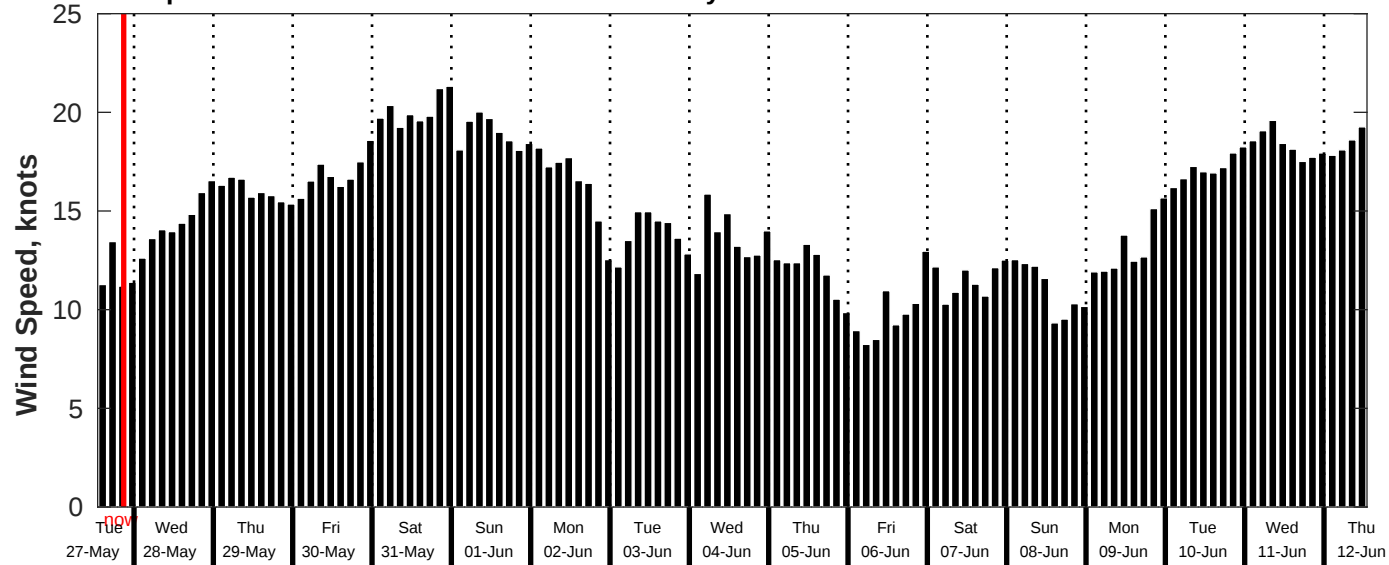
GFS Wind Speed Forecast for NDBC 51209 from 27-May-2025 13:00:00 to 12-Jun-2025 13:00:00
