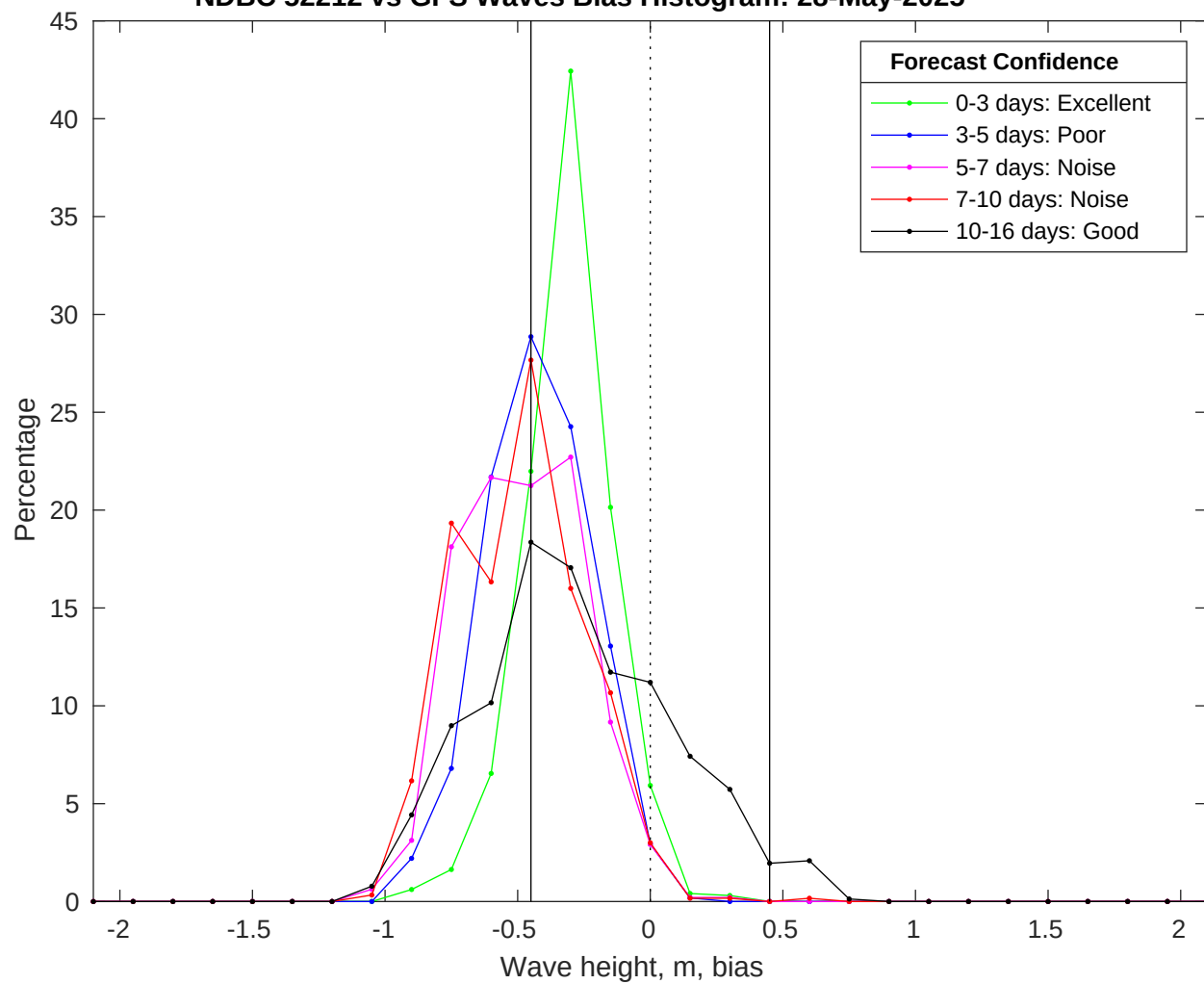
NDBC 52212 vs GFS Waves Bias Histogram: 28-May-2025
