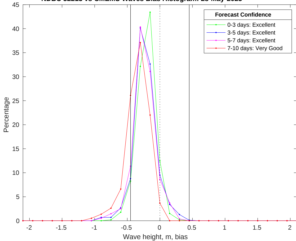
NDBC 52213 vs CMEMS Waves Bias Histogram: 28-May-2025
