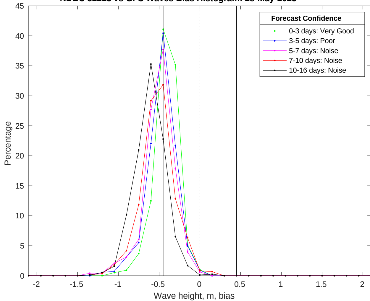
NDBC 52213 vs GFS Waves Bias Histogram: 28-May-2025
