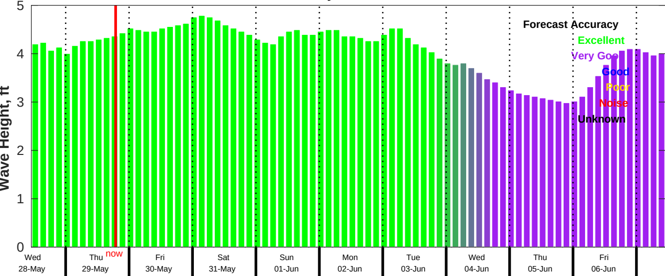
CMEMS Wave Forecast for NDBC 52213 from 27-May-2025 11:00:00 to 06-Jun-2025 11:00:00
