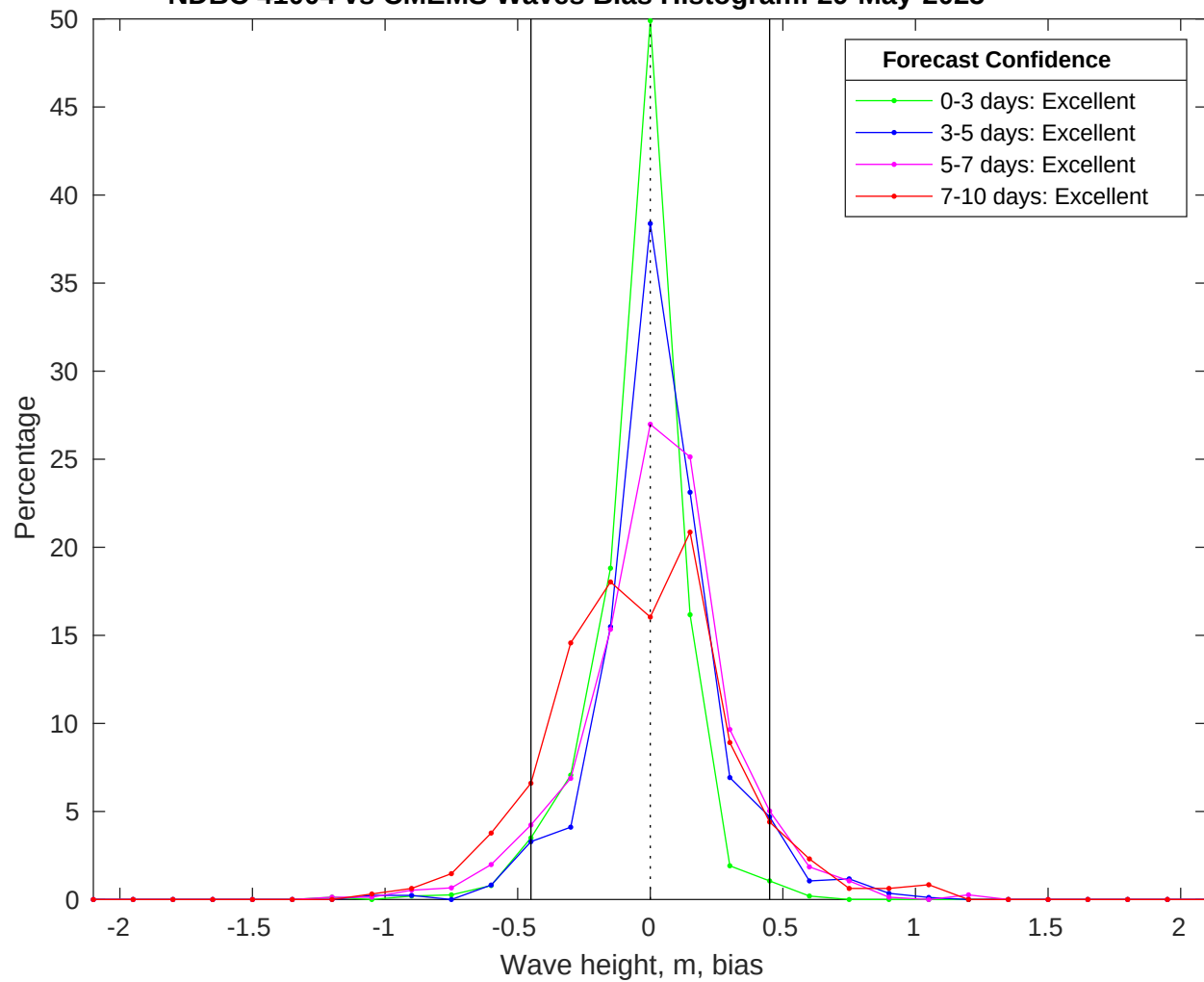
NDBC 41004 vs CMEMS Waves Bias Histogram: 29-May-2025
