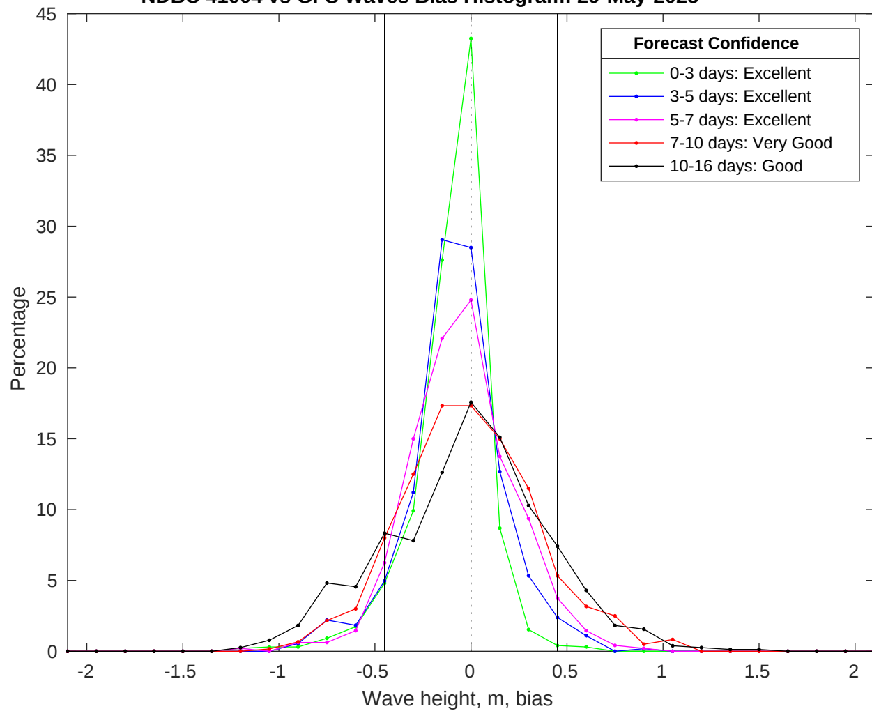
NDBC 41004 vs GFS Waves Bias Histogram: 29-May-2025
