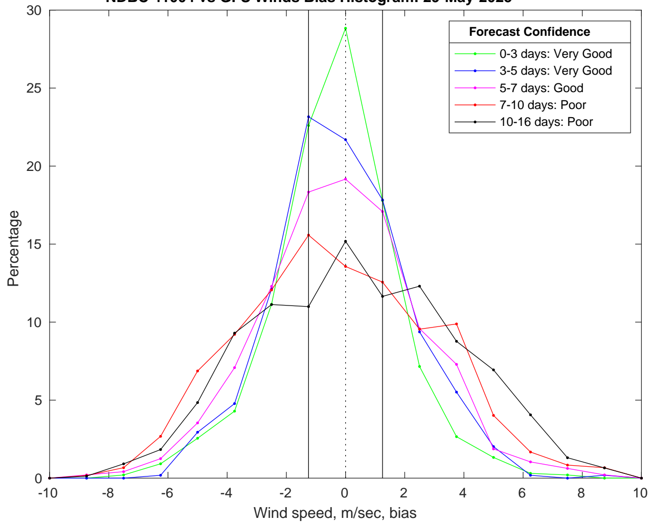
NDBC 41004 vs GFS Winds Bias Histogram: 29-May-2025
