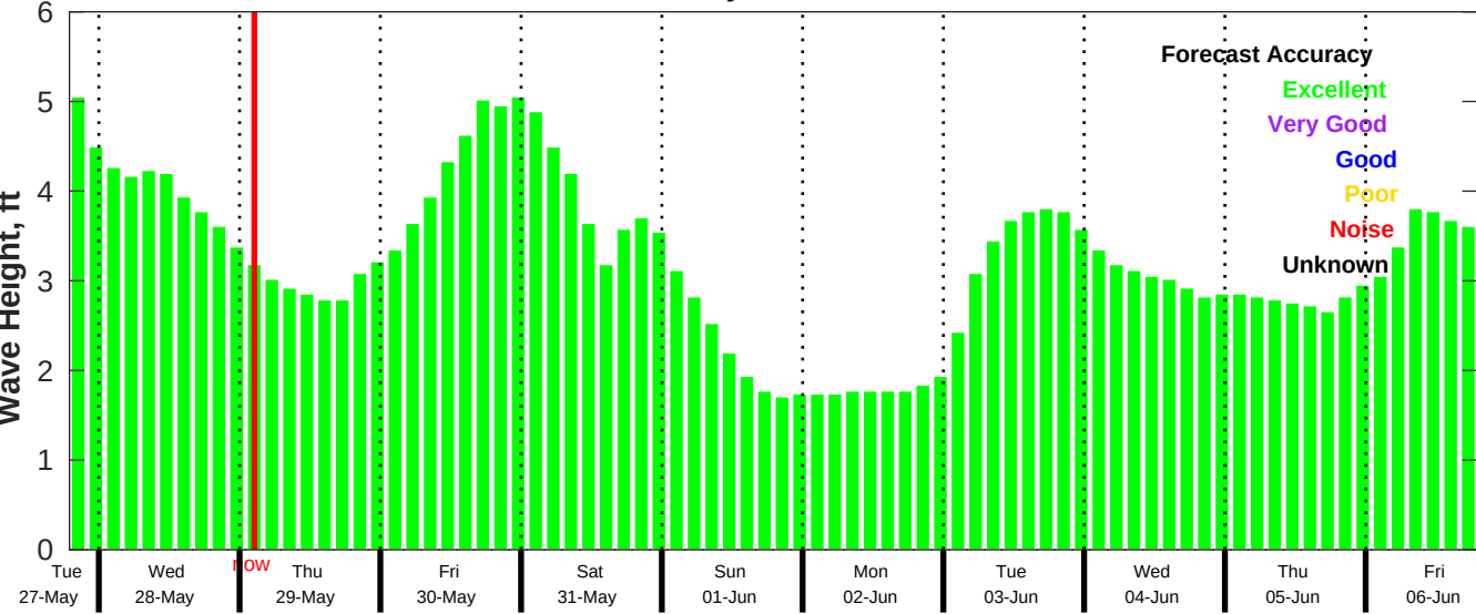
CMEMS Wave Forecast for NDBC 41004 from 27-May-2025 19:00:00 to 06-Jun-2025 19:00:00
