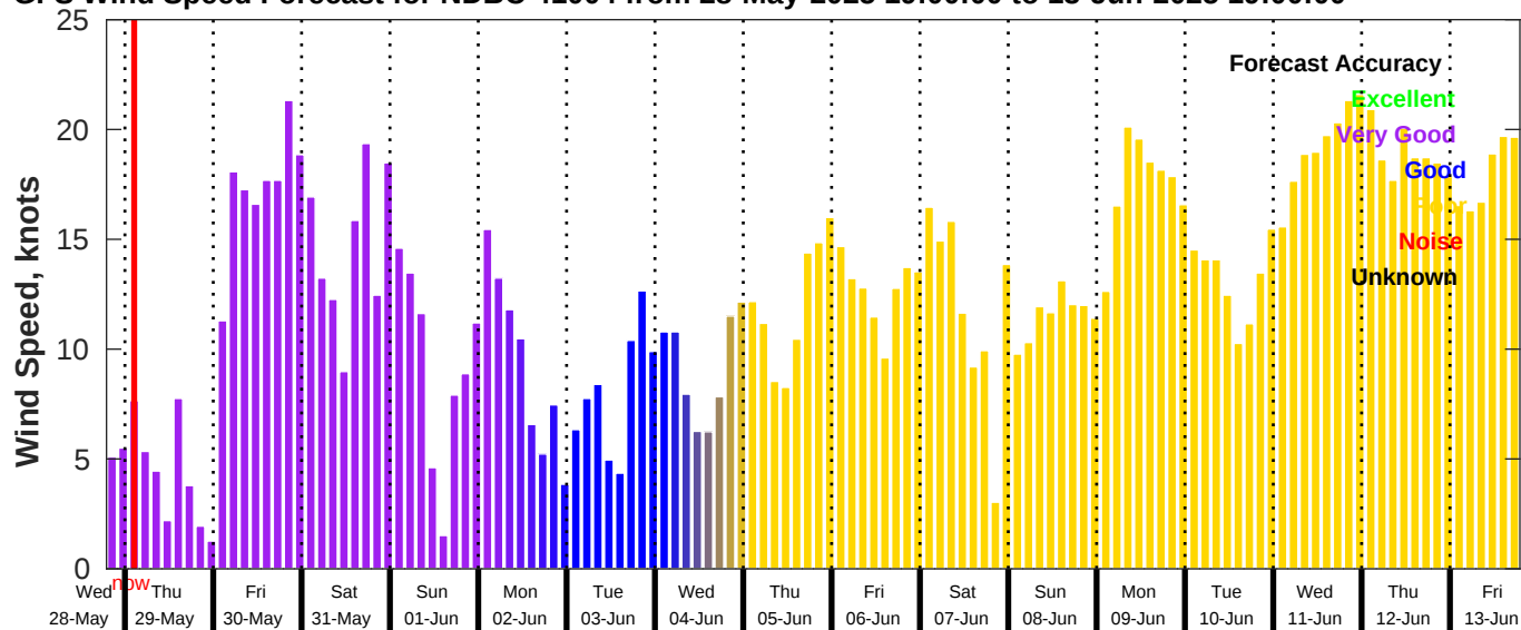
GFS Wind Speed Forecast for NDBC 41004 from 28-May-2025 19:00:00 to 13-Jun-2025 19:00:00
