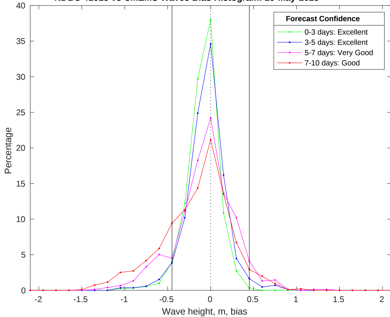
NDBC 41013 vs CMEMS Waves Bias Histogram: 29-May-2025
