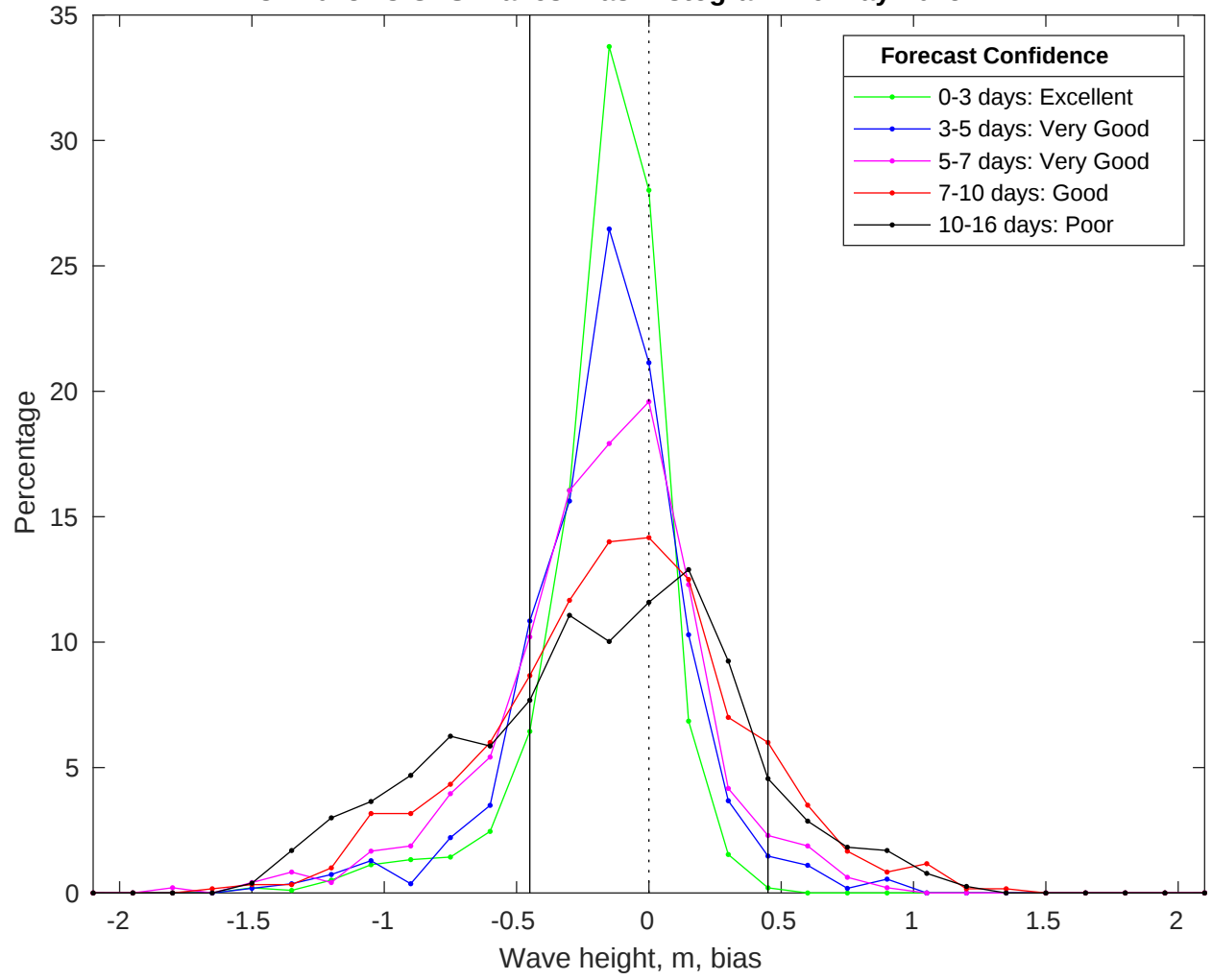
NDBC 41013 vs GFS Waves Bias Histogram: 29-May-2025
