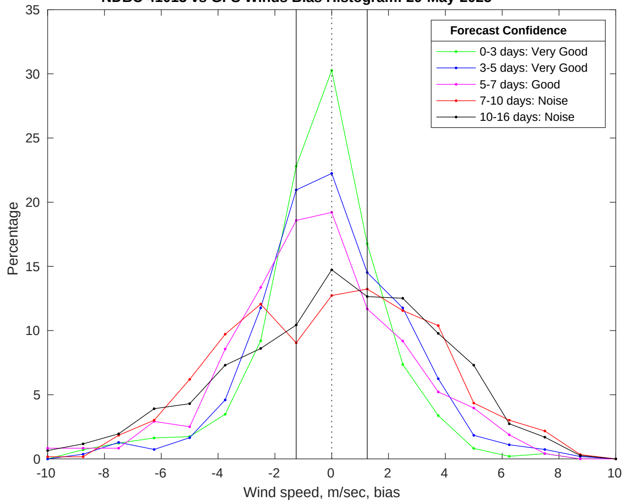
NDBC 41013 vs GFS Winds Bias Histogram: 29-May-2025
