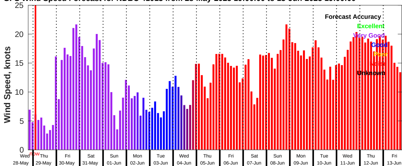
GFS Wind Speed Forecast for NDBC 41013 from 28-May-2025 19:00:00 to 13-Jun-2025 19:00:00
