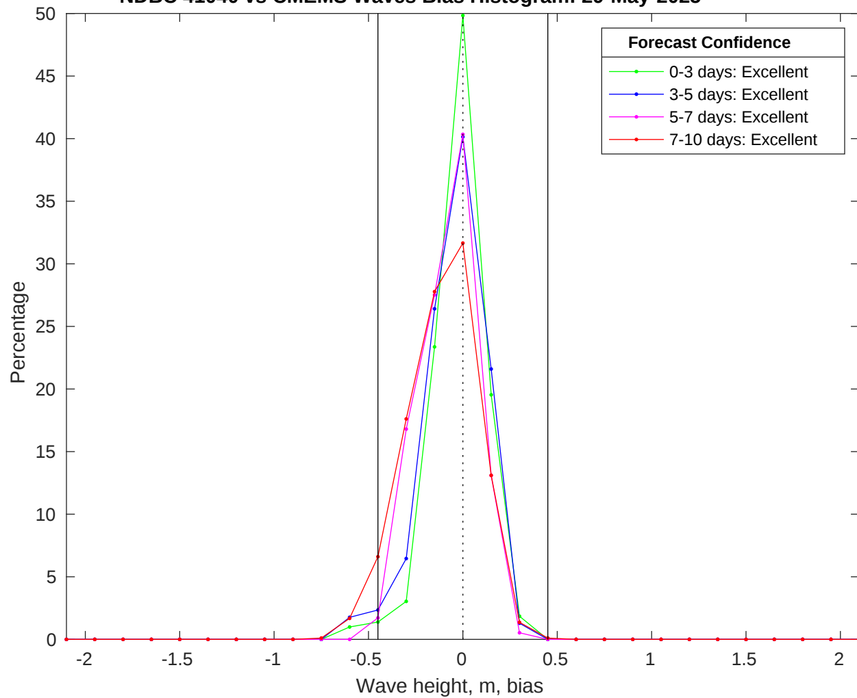
NDBC 41040 vs CMEMS Waves Bias Histogram: 29-May-2025
