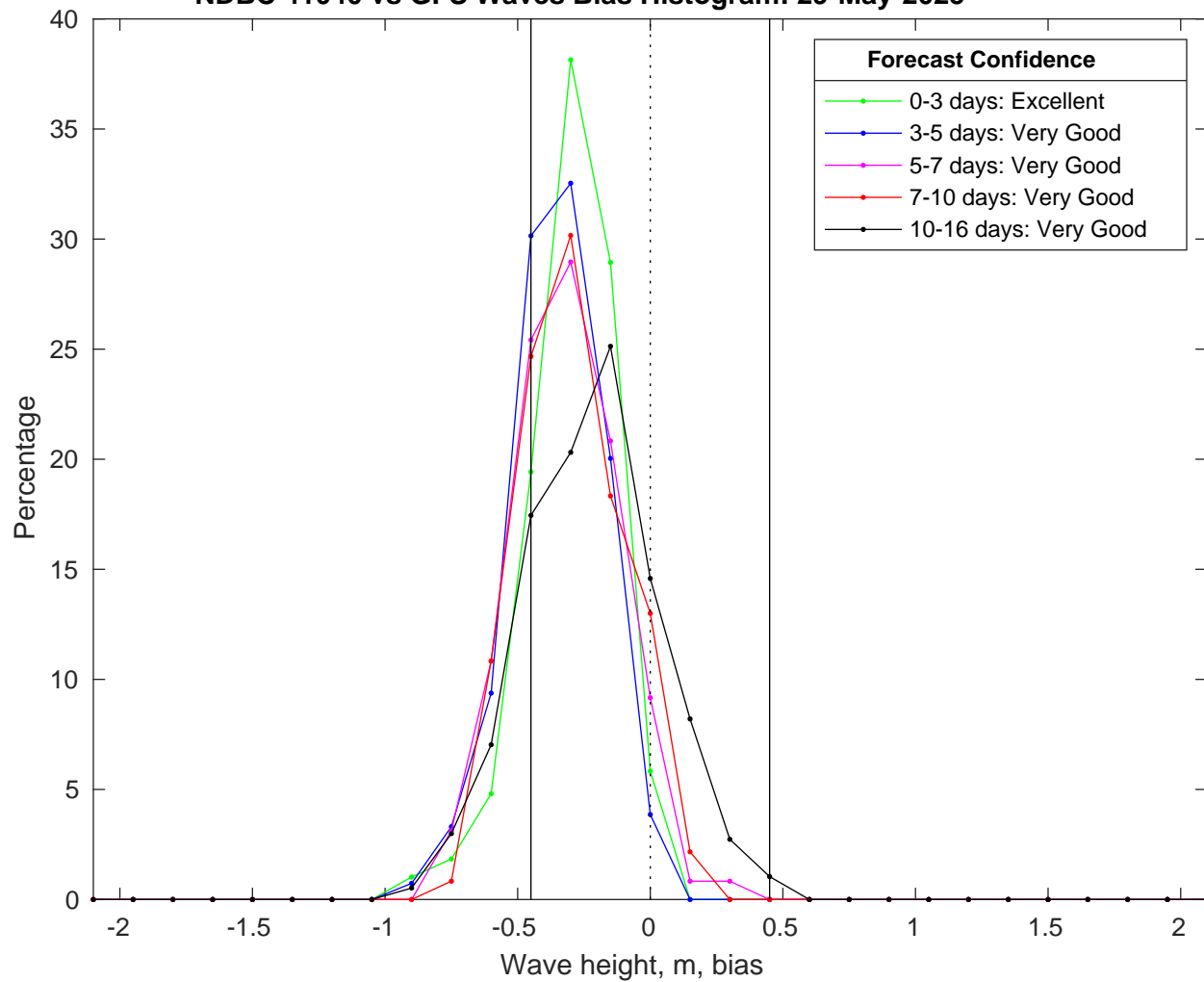
NDBC 41040 vs GFS Waves Bias Histogram: 29-May-2025
