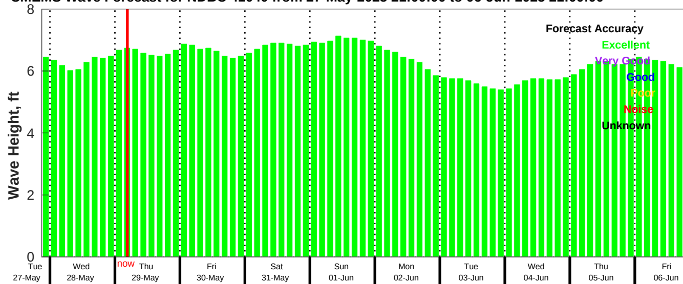
CMEMS Wave Forecast for NDBC 41040 from 27-May-2025 21:00:00 to 06-Jun-2025 21:00:00
