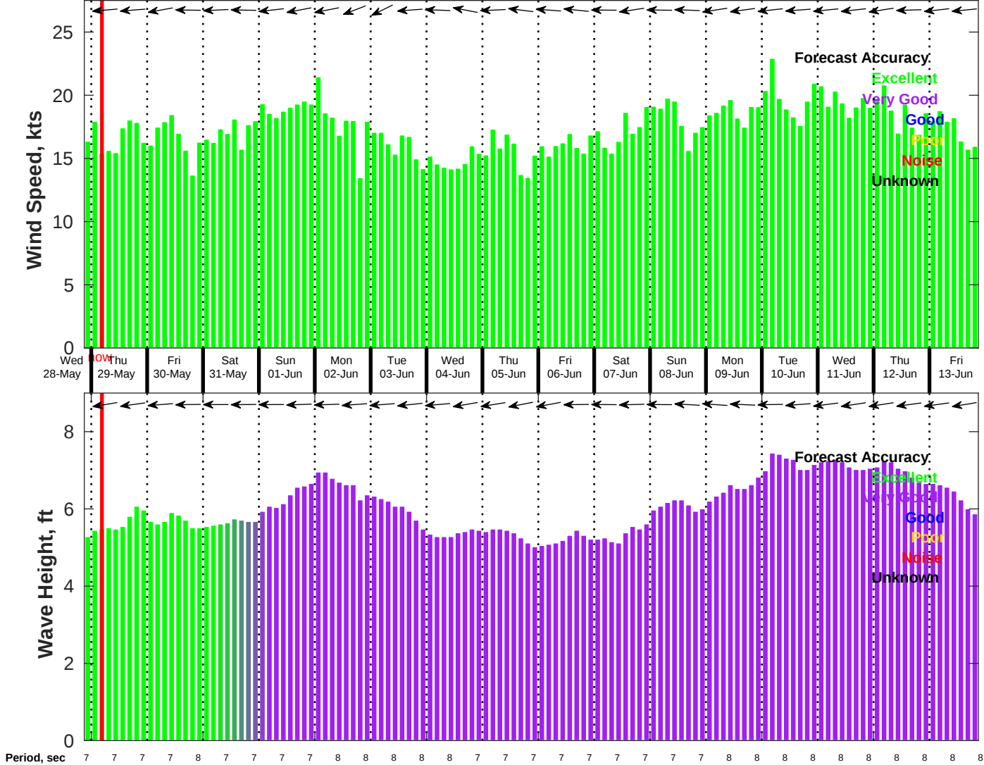
Wind & Wave Forecast for NDBC 41040 from 28-May-2025 21:00:00 to 13-Jun-2025 21:00:00
