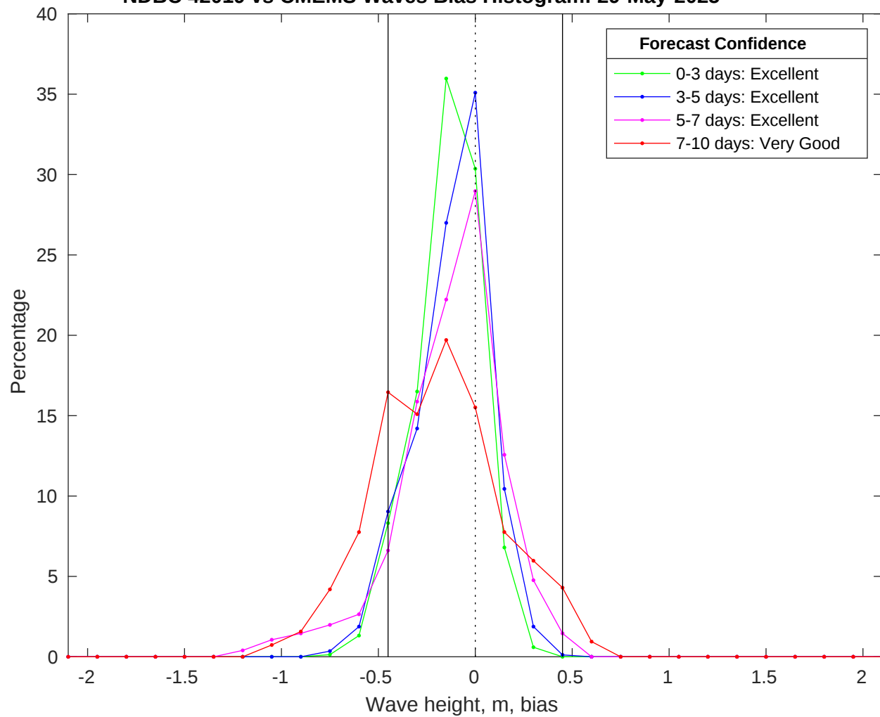
NDBC 42019 vs CMEMS Waves Bias Histogram: 29-May-2025
