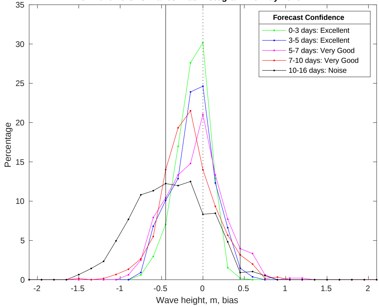
NDBC 42019 vs GFS Waves Bias Histogram: 29-May-2025
