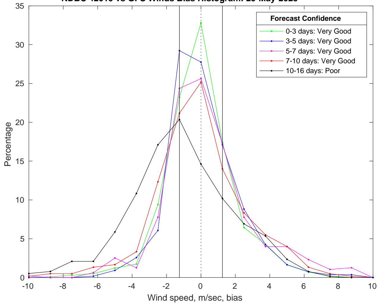
NDBC 42019 vs GFS Winds Bias Histogram: 29-May-2025
