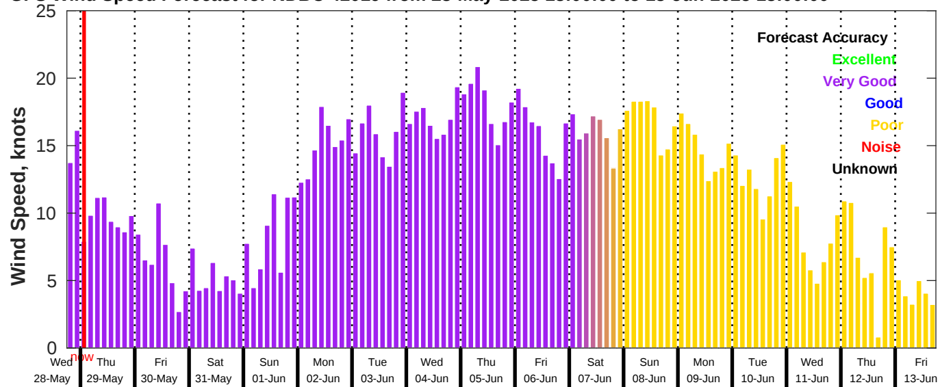
GFS Wind Speed Forecast for NDBC 42019 from 28-May-2025 18:00:00 to 13-Jun-2025 18:00:00
