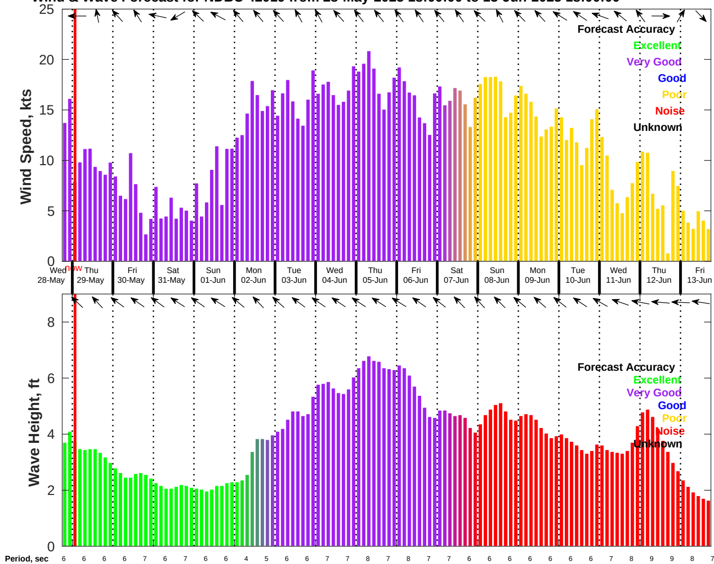
Wind & Wave Forecast for NDBC 42019 from 28-May-2025 18:00:00 to 13-Jun-2025 18:00:00
