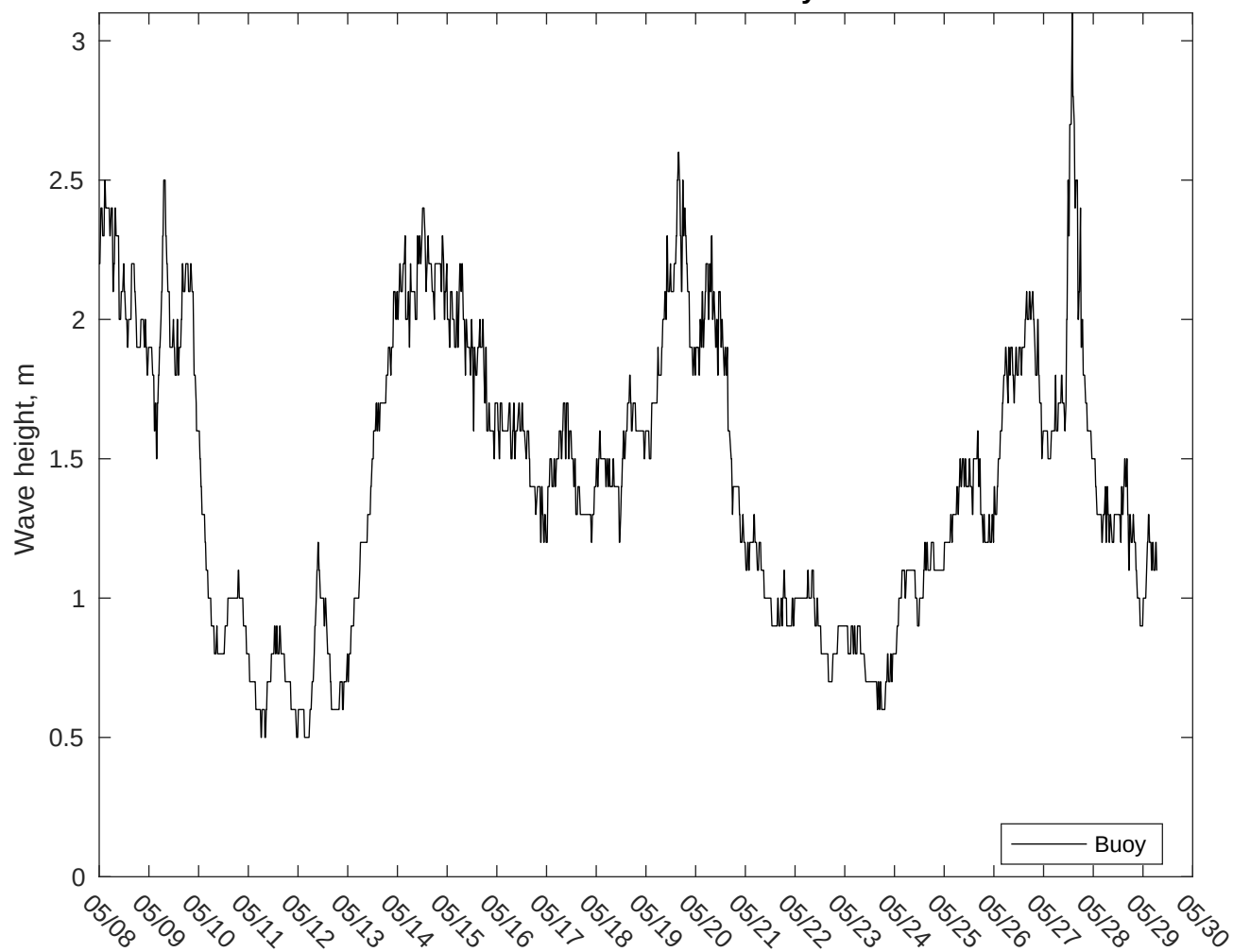
NDBC 42020 vs CMEMS Waves: 10 to 16 day forecast
