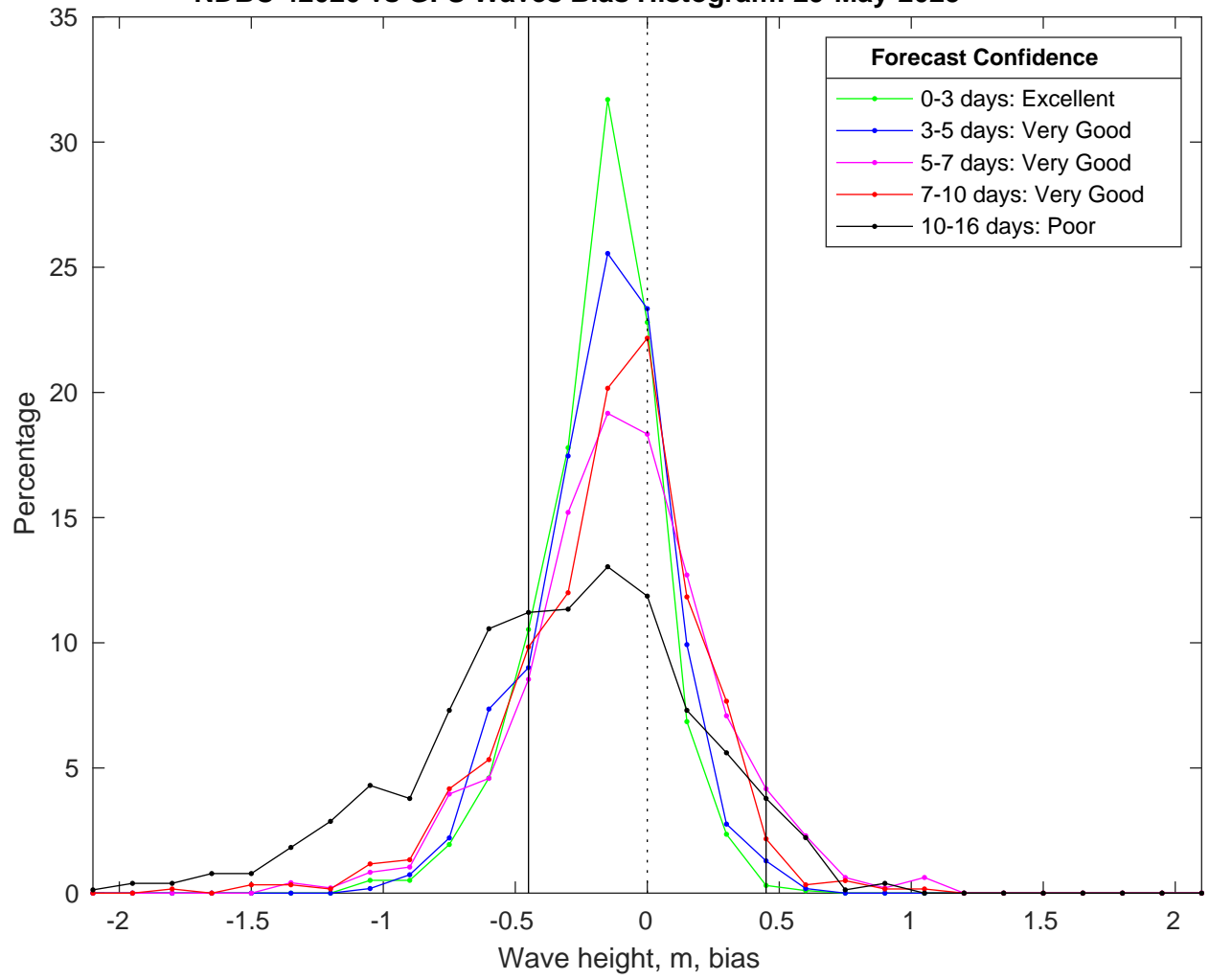
NDBC 42020 vs GFS Waves Bias Histogram: 29-May-2025
