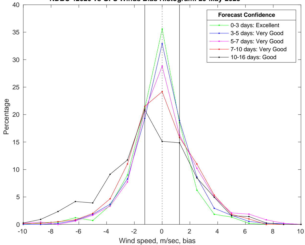
NDBC 42020 vs GFS Winds Bias Histogram: 29-May-2025
