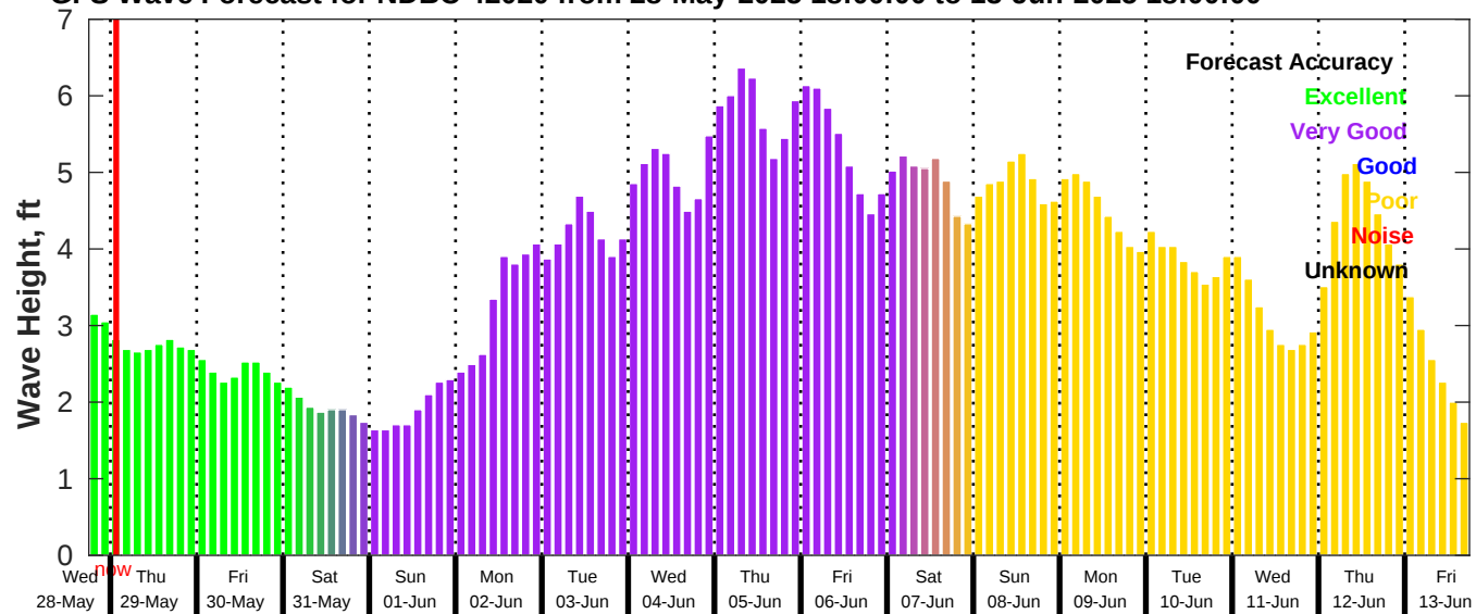
GFS Wave Forecast for NDBC 42020 from 28-May-2025 18:00:00 to 13-Jun-2025 18:00:00
