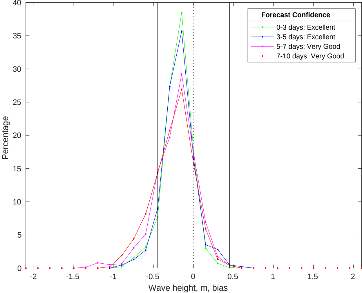
NDBC 42035 vs CMEMS Waves Bias Histogram: 29-May-2025
