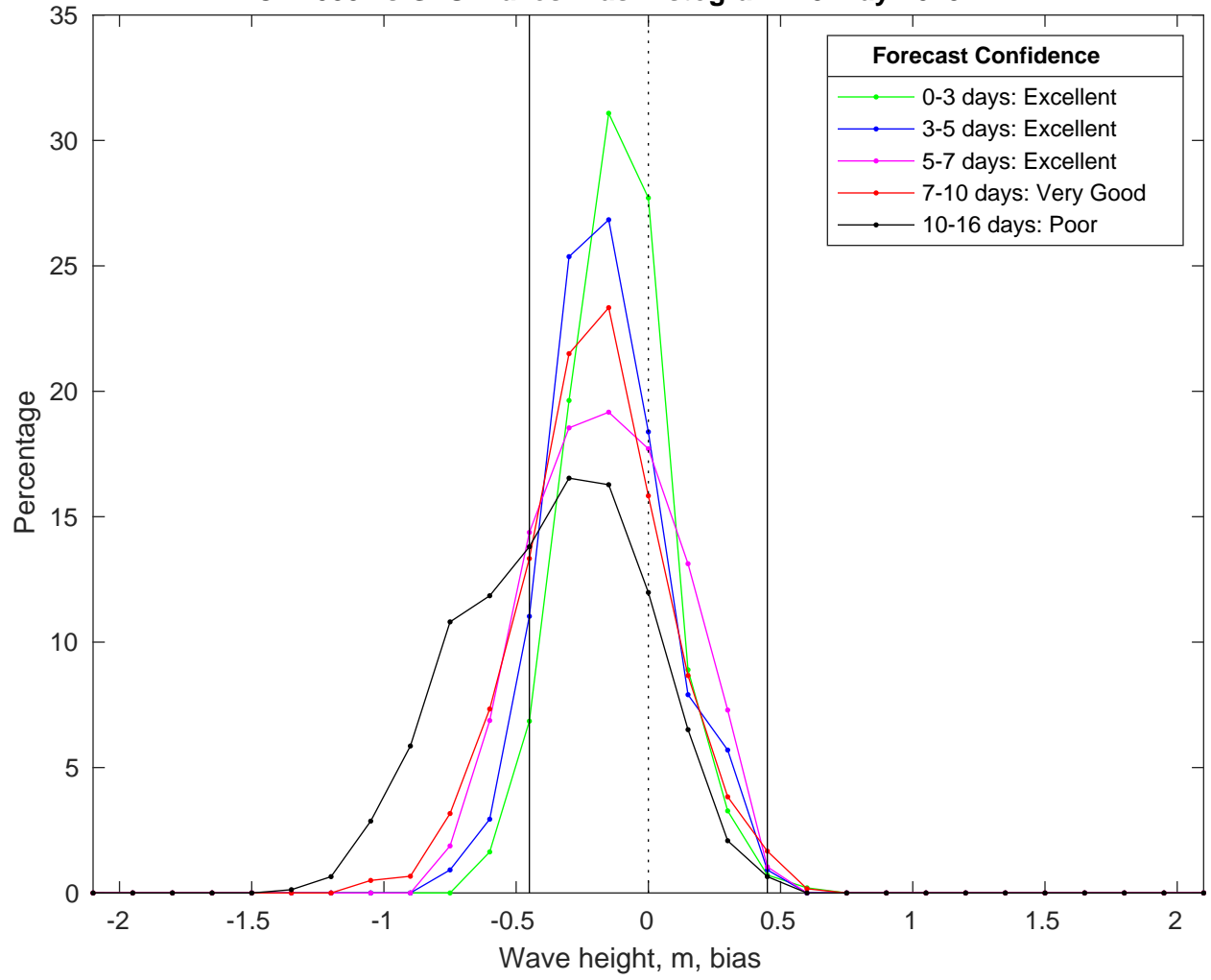
NDBC 42035 vs GFS Waves Bias Histogram: 29-May-2025
