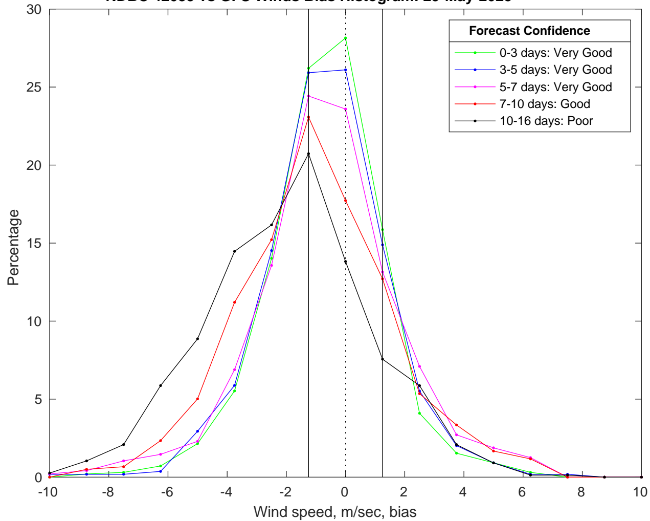
NDBC 42035 vs GFS Winds Bias Histogram: 29-May-2025
