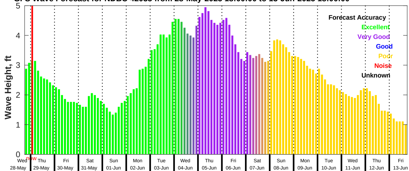
GFS Wave Forecast for NDBC 42035 from 28-May-2025 18:00:00 to 13-Jun-2025 18:00:00
