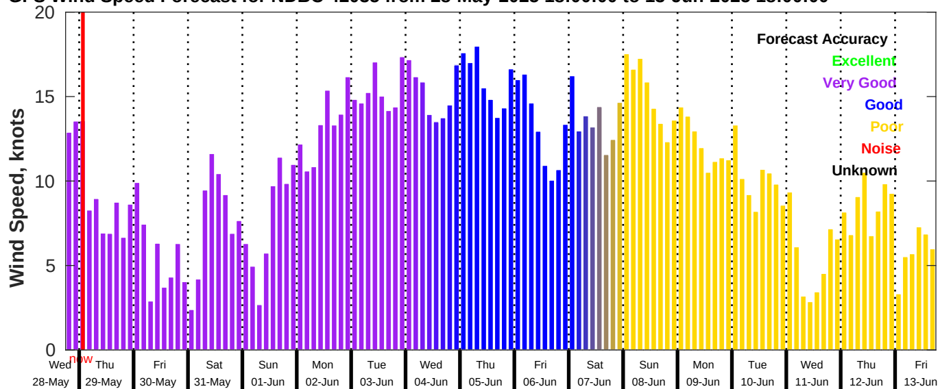
GFS Wind Speed Forecast for NDBC 42035 from 28-May-2025 18:00:00 to 13-Jun-2025 18:00:00
