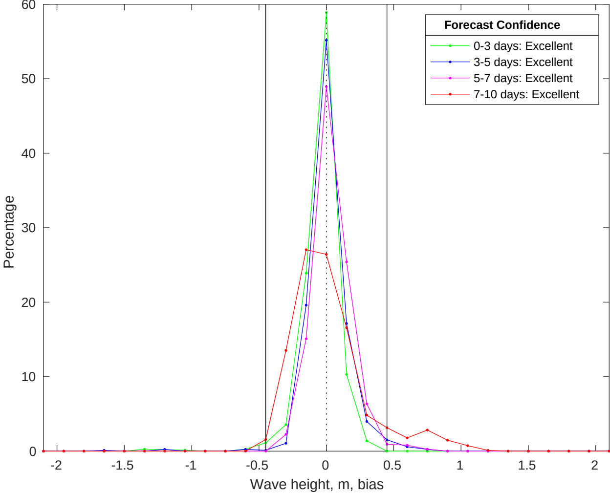
NDBC 42036 vs CMEMS Waves Bias Histogram: 29-May-2025
