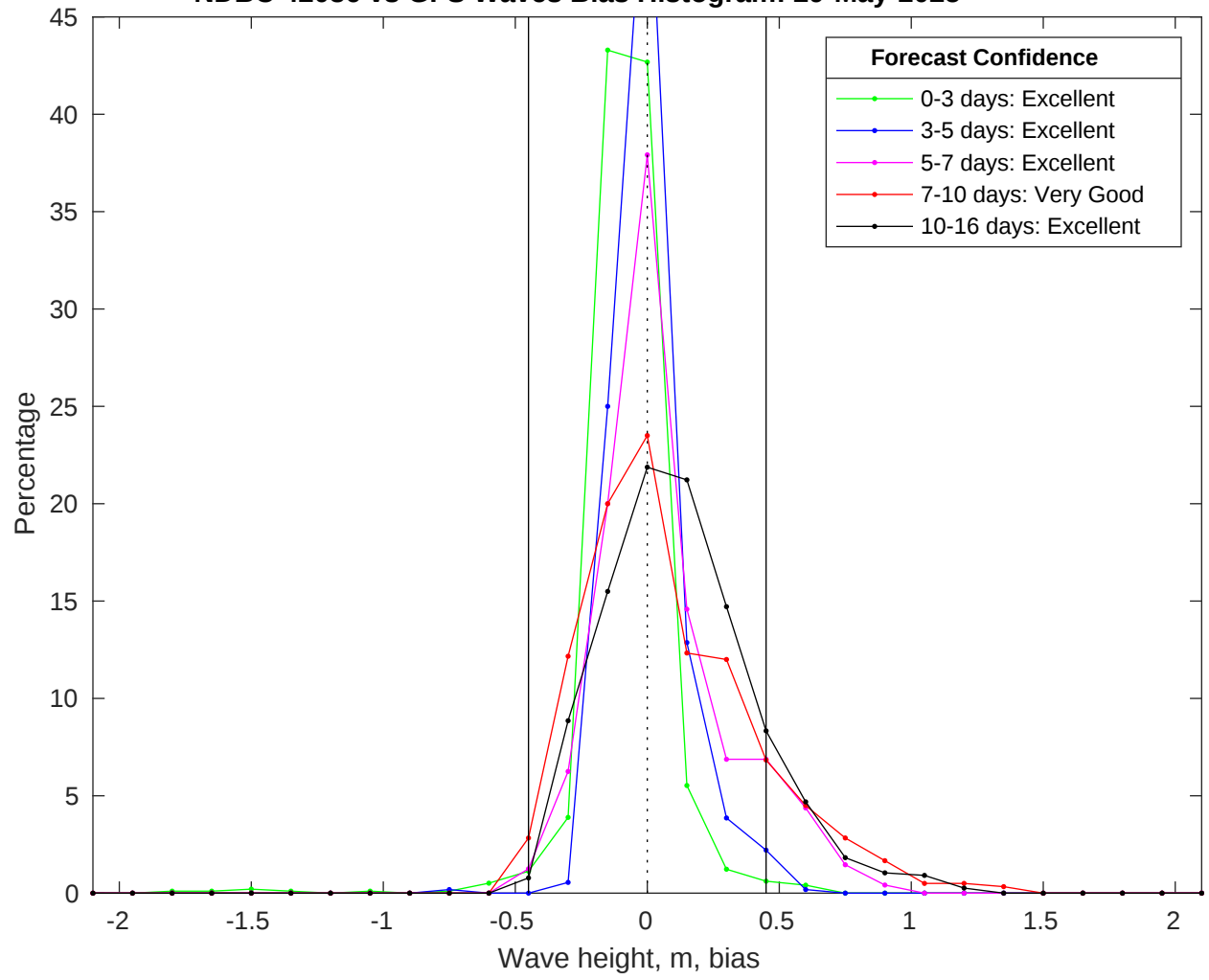
NDBC 42036 vs GFS Waves Bias Histogram: 29-May-2025
