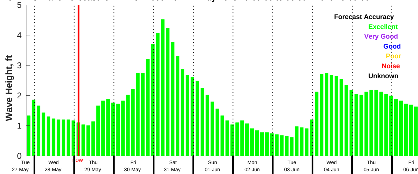
CMEMS Wave Forecast for NDBC 42036 from 27-May-2025 19:00:00 to 06-Jun-2025 19:00:00
