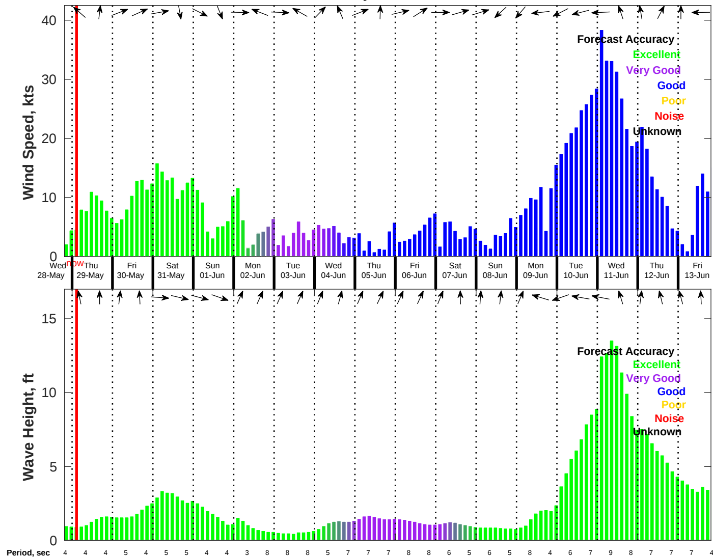
Wind & Wave Forecast for NDBC 42036 from 28-May-2025 19:00:00 to 13-Jun-2025 19:00:00
