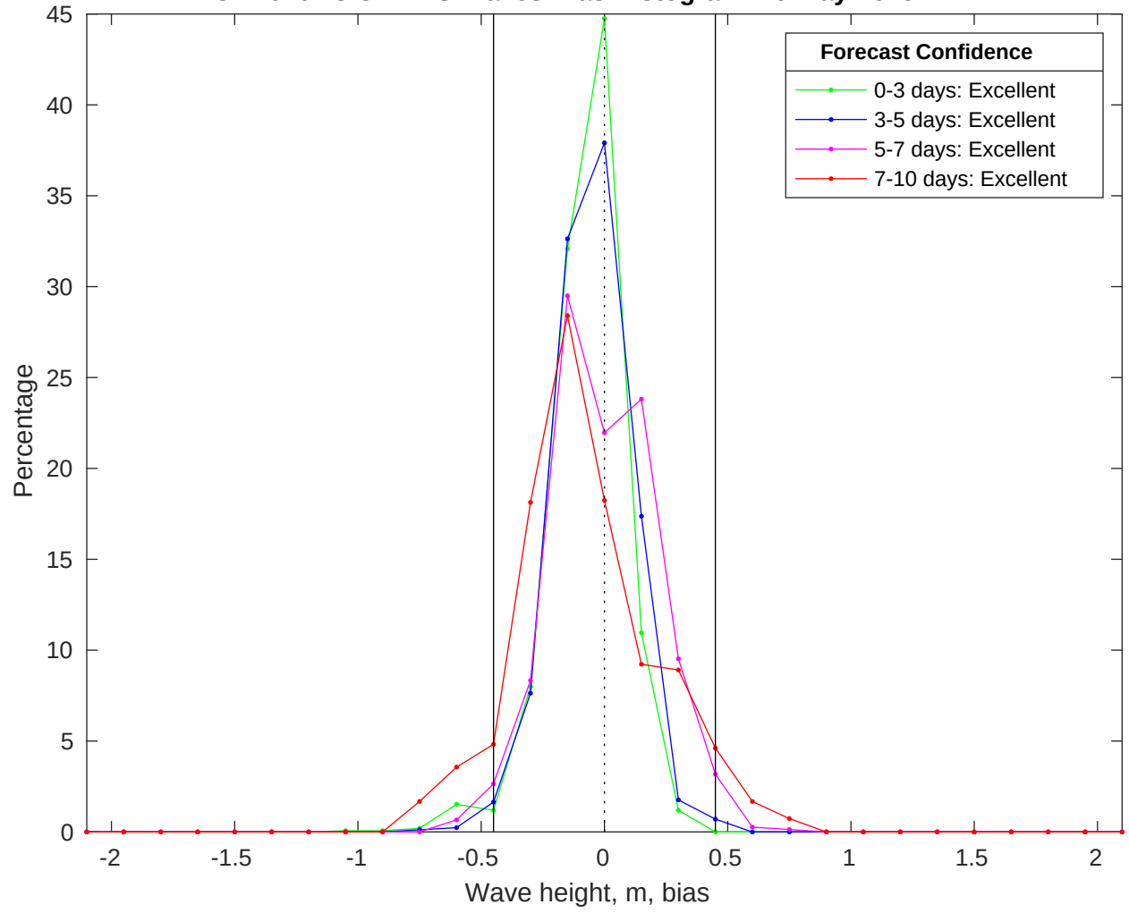
NDBC 42040 vs CMEMS Waves Bias Histogram: 29-May-2025
