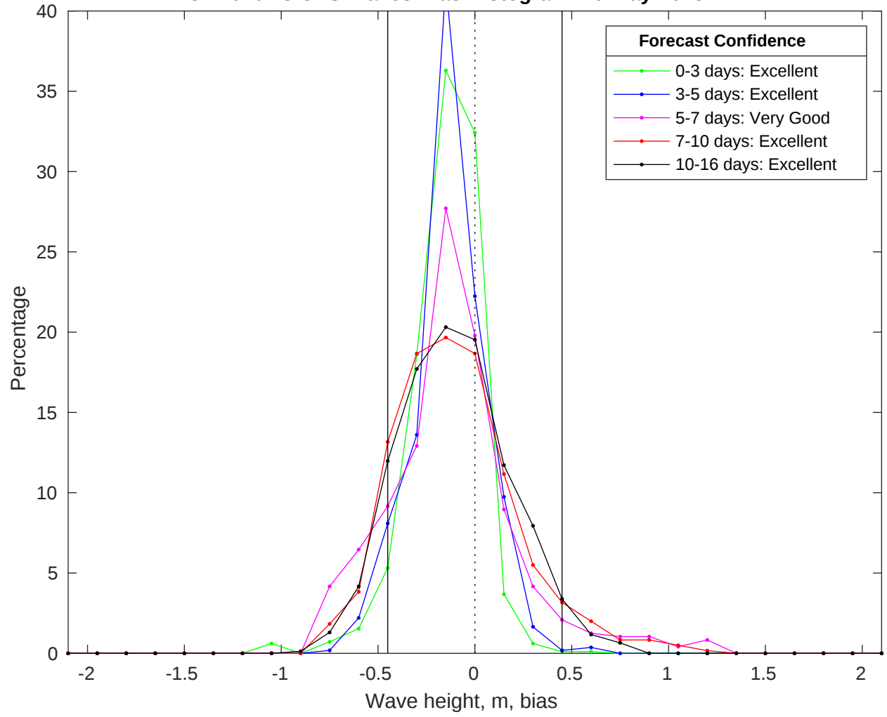
NDBC 42040 vs GFS Waves Bias Histogram: 29-May-2025
